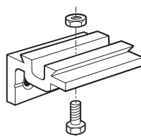
Soporte pared 6 mm Wall bracket 1/4"
