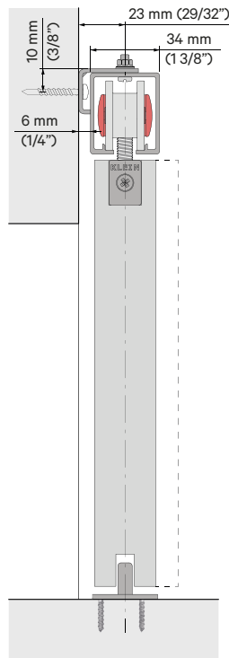
Perfil Soporte 6mm | Wall Support Profile 6 mm | Profil de Support 6 mm Perfil Soporte 17 mm | Wall Support Profile 17 mm | Profil de Support 17 mm
