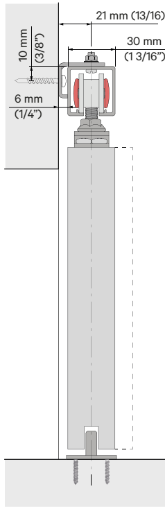
Perfil Soporte 6mm | Wall Support Profile 6 mm | Profil de Support 6 mm Perfil Soporte 17 mm | Wall Support Profile 17 mm | Profil de Support 17 mm
