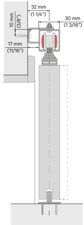
Perfil Soporte 6mm | Wall Support Profile 6 mm | Profil de Support 6 mm Perfil Soporte 17 mm | Wall Support Profile 17 mm | Profil de Support 17 mm
